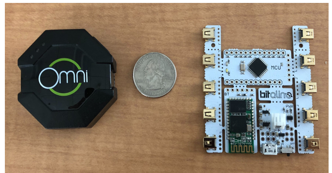
Figure 3: The Omni IMU Pod clips to the front of the shoe to allow for natural movement and gait [left]. Bitalino board is attached to a belt around the user and does not prohibit movement [right]
