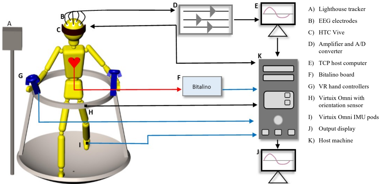
Figure 1: Top-level block diagram of the IMAS system. The user ambulates in a 360 degree treadmill while participating in a virtual foot patrol. Movement kinematics and biomedical signals are recorded for post-hoc analysis.
